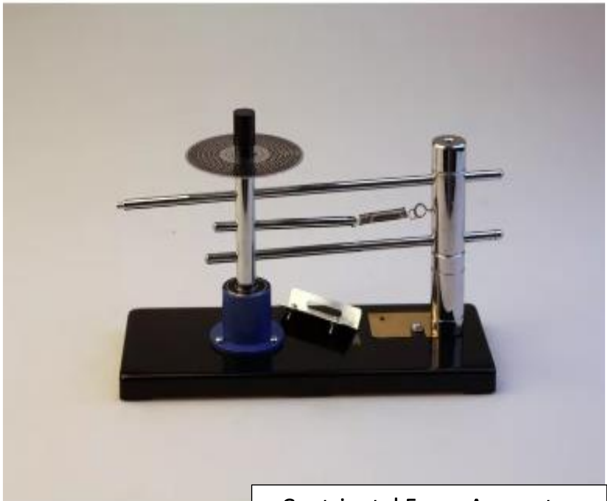
Centripetal Force Apparatus
